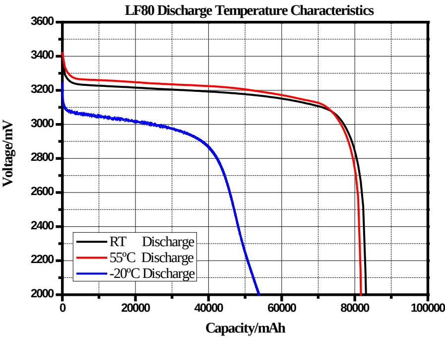
Fig.2 Different temperature discharge curve
